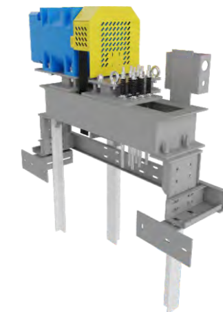
Machine- Room-Less drive-frame guide rail
